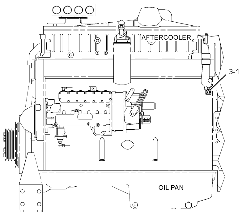
LEFT SIDE VIEW OF ENGINE
